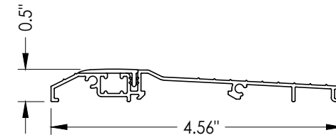
T13 INSWING/OUTSWING ACCESSIBLE THRESHOLD ADAPI4562 / ADAPO4562
