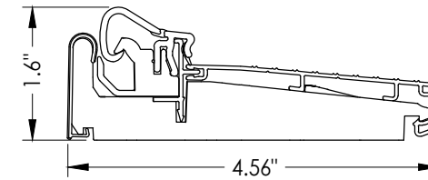
T8 INSWING ARTICULATING THRESHOLD ZAC4565RDS
